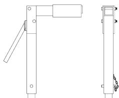
JKL1 - Breakover Jackleg
