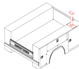
Hydraulic Out, Hydraulic Down
